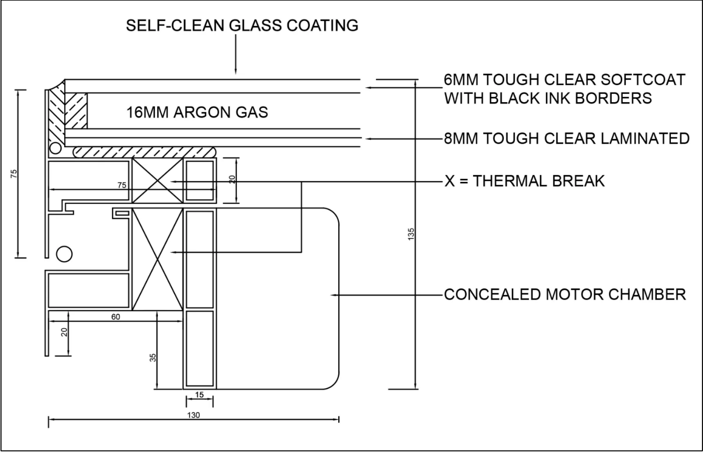
Technical Drawing 1
