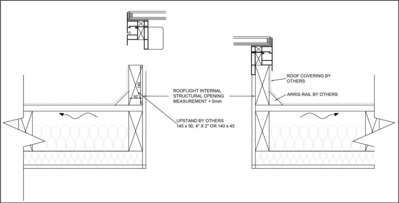
Installation Upstand Detail Drawing 2
